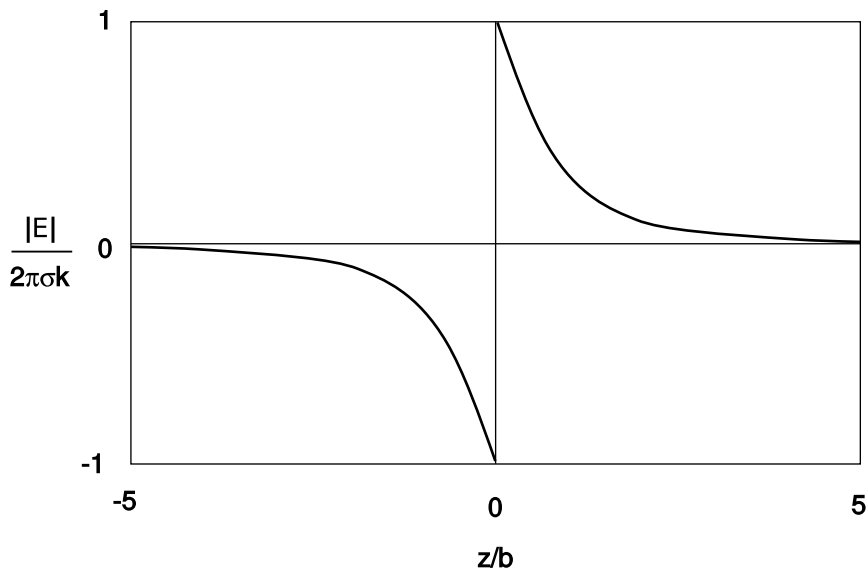
g / Example 13: variation of the field ( \sigma > 0 ).
